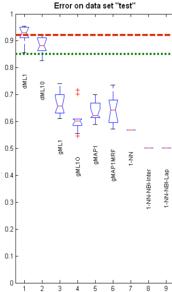
Fig. 3. Comparison of KNN and KNN+NBIC against semi-supervised methods in [4, 5, 3, 11]; error is measured at the first label. We used the parameter configurations described in Table 3.
