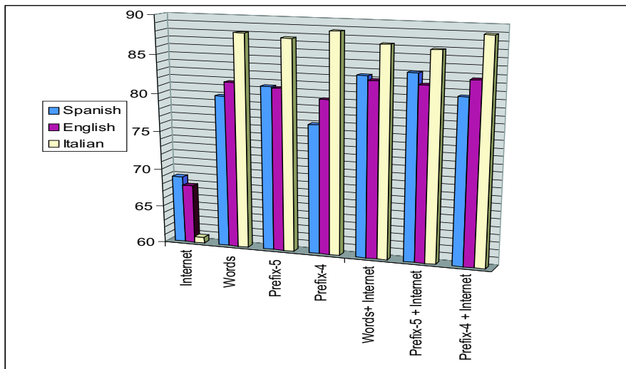
Figure 1: Graphical comparison of question classification accuracies
