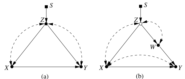
FIG. 5. Selection diagrams illustrating S -admissibility. (a) Has no S -admissible set while in (b), W is S -admissible.
