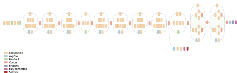
Fig. 4: Inception v3 general architecture
