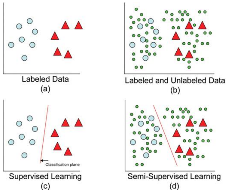
Figure: https://www.digitalvidya.com/blog/semi-supervised-learning/
